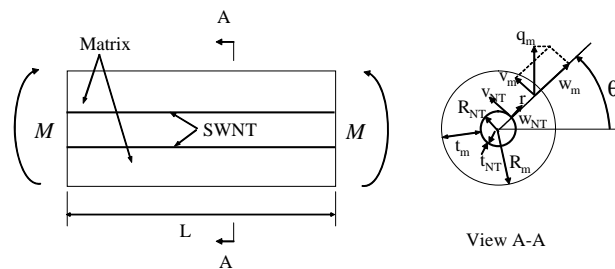
Fig. 1. Nanocomposite beam geometry, where L is the length; R_{\text{NT}} and R_{\text{m}} are the original radius of the SWNT and the original outer radius of the matrix, respectively; t_{\text{NT}} is the wall thickness of the SWNT; v and w are the radial and circumferential displacements at a material point, 'NT' refers to the SWNT and 'm' refers to the matrix; r is the radial coordinate, \theta is the circumferential coordinate and M is the external bending moment.
